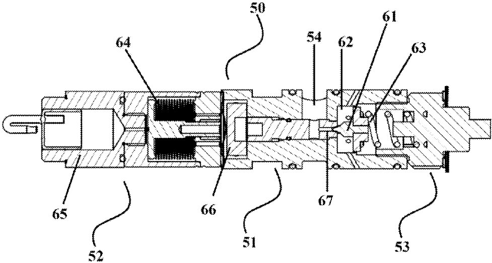
Figure 6: Section A-A View of the TXV Cartridge
