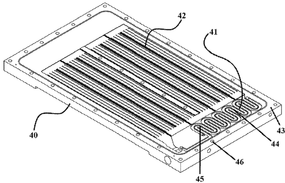
Figure 4: Alternative embodiment of the Current Invention of Integrating the TXV and Sensing Bulb within Each of Plurality of Evaporative Cold Plates with a recuperative heat exchanger.
