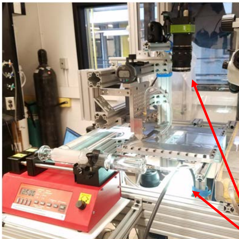
Georgia Tech's coating line (mounted above)
